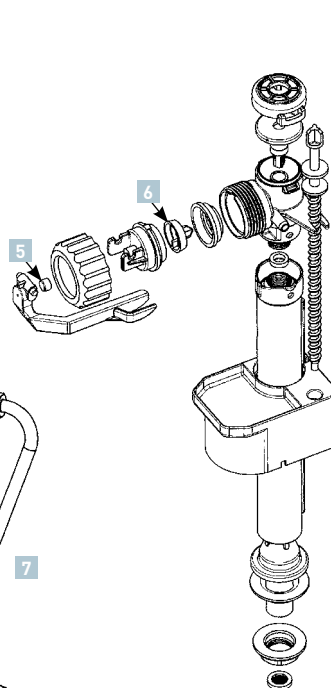
COMPACT 99B
