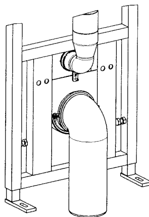
Bend outlet
